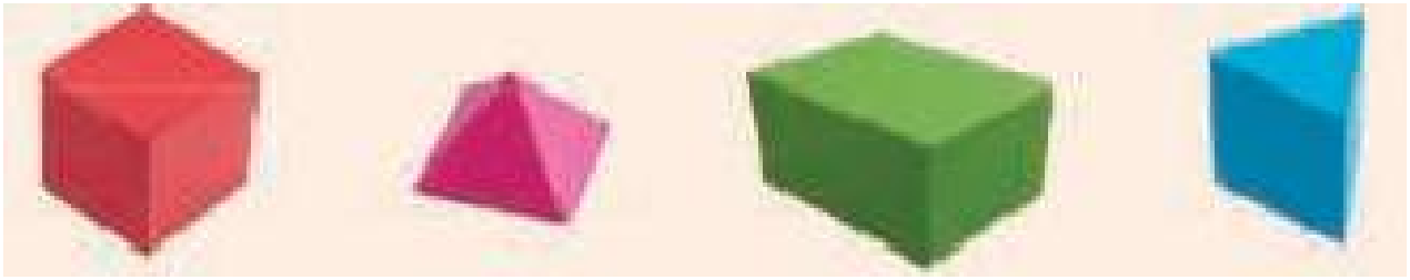
Cube (a)
